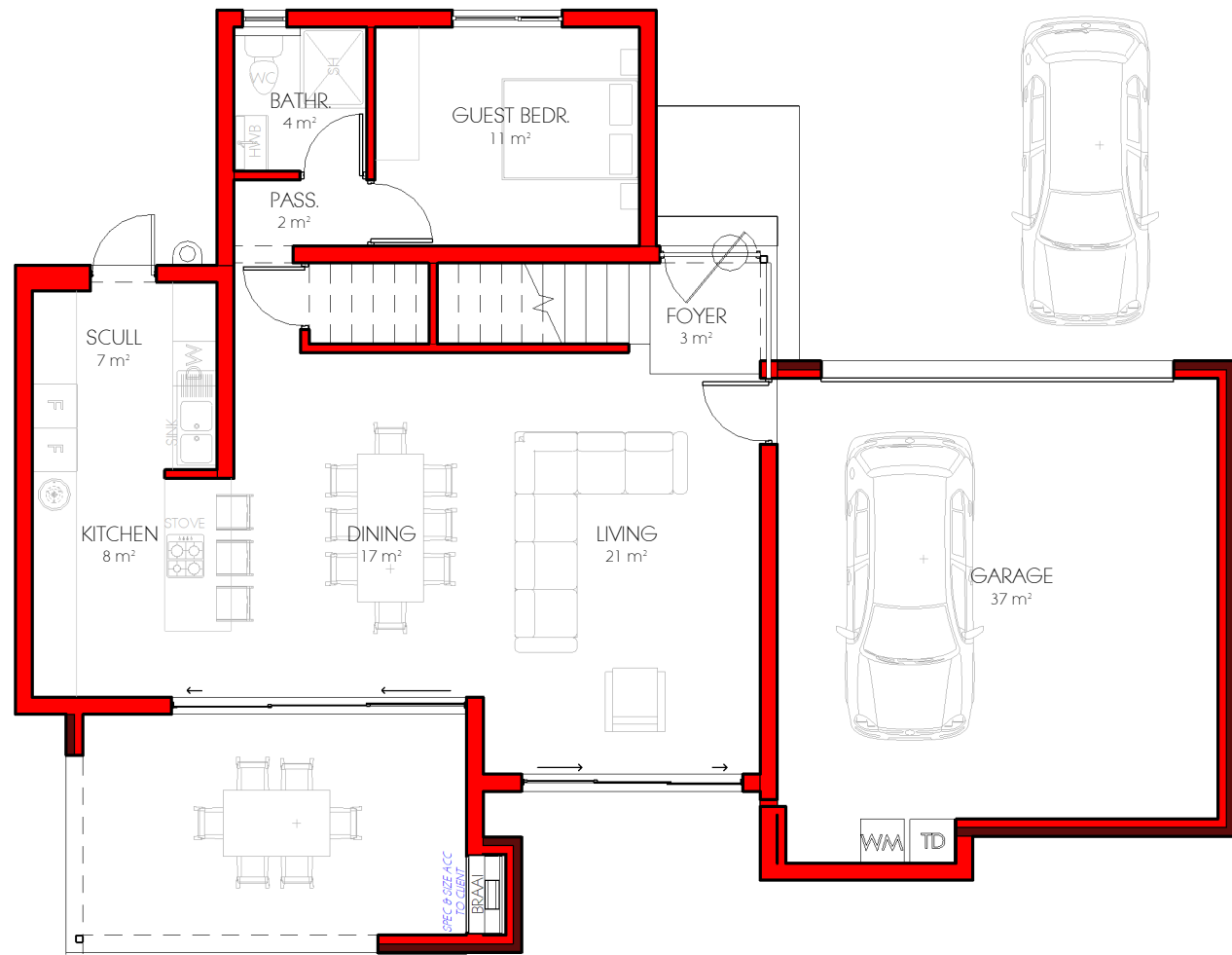
02 GROUND FLOOR. 1 : 100
