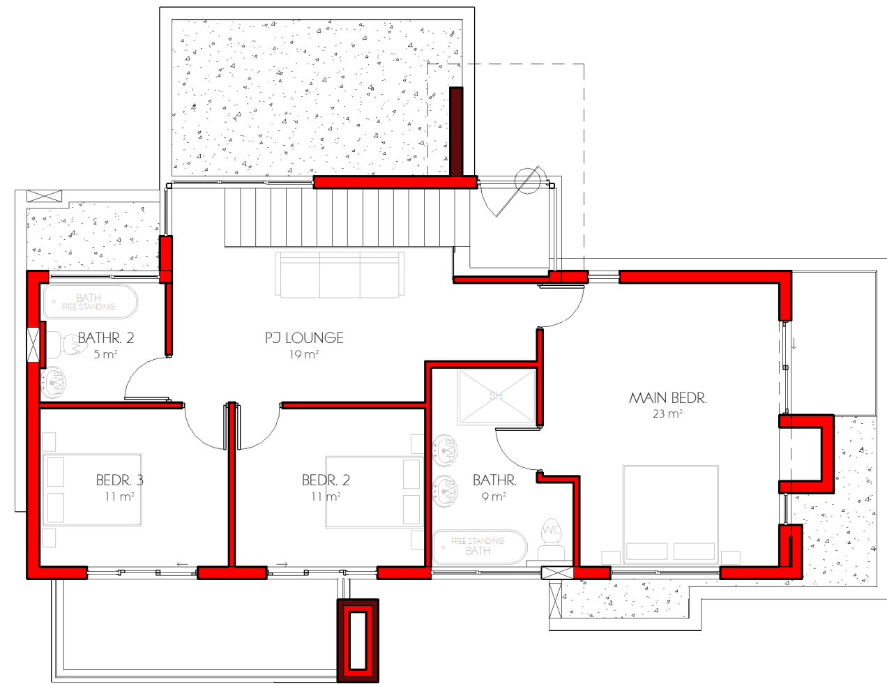
03 FIRST FLOOR. 1 : 100
