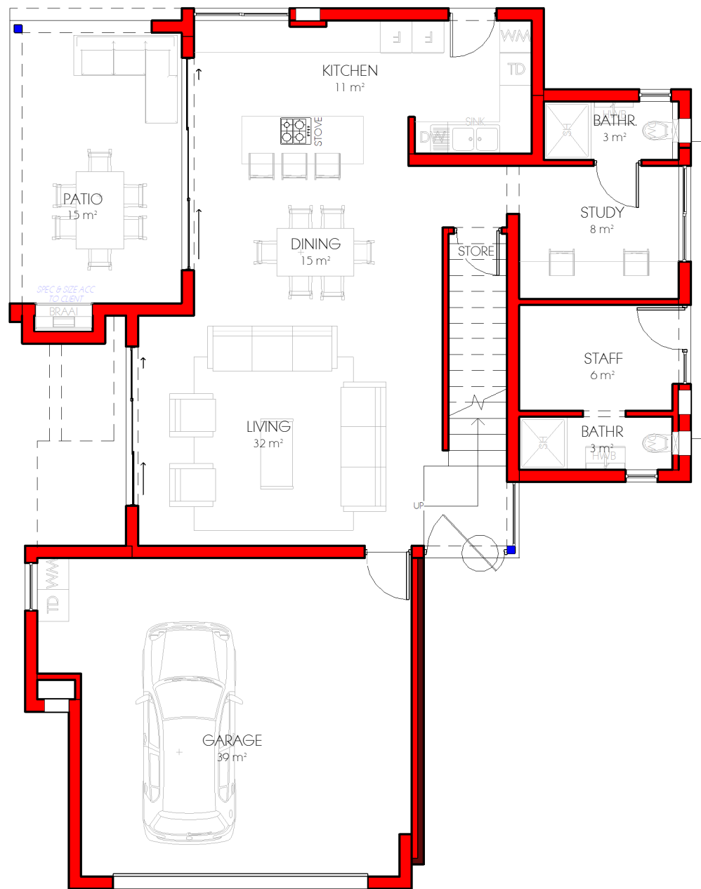
02 GROUND FLOOR 1 : 100
