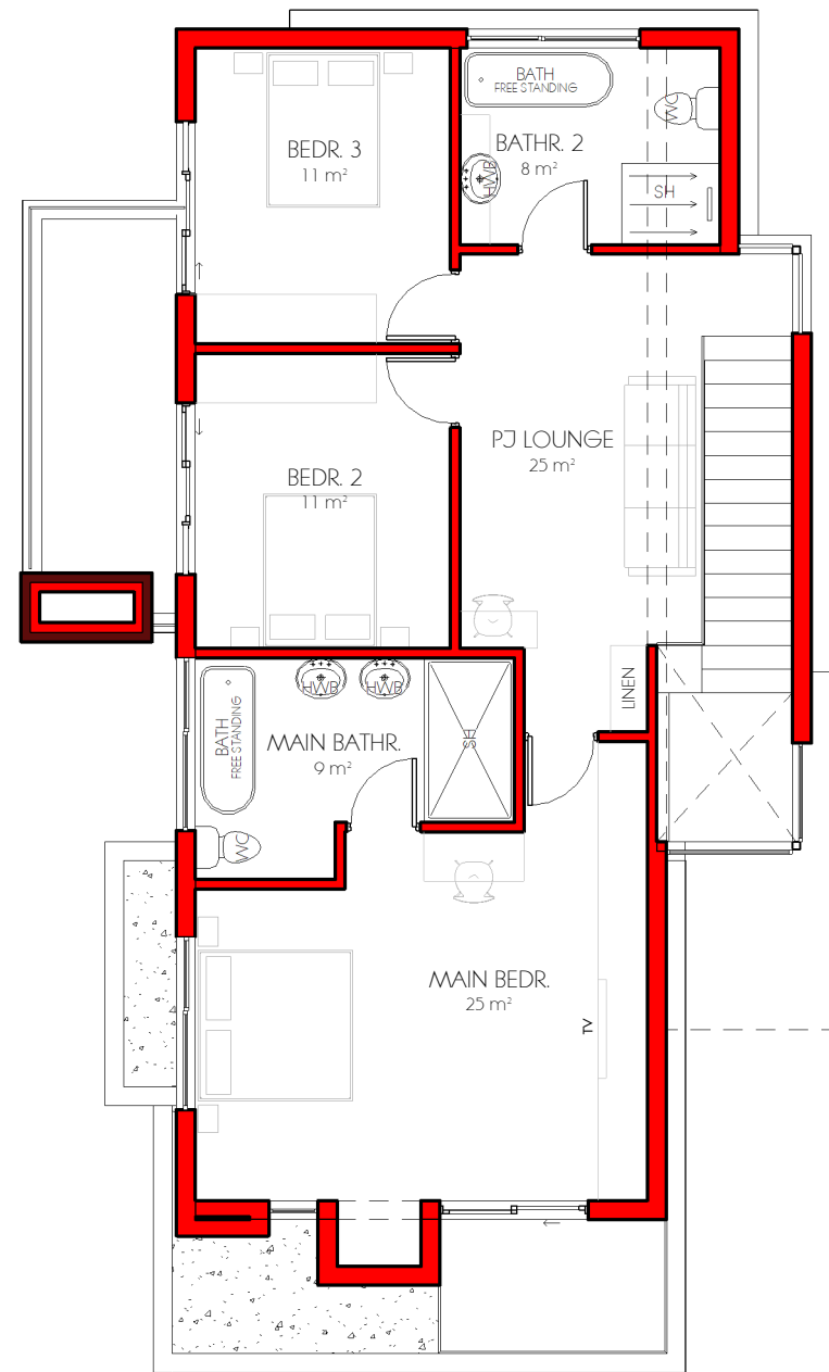
03 FIRST FLOOR 1 : 100
