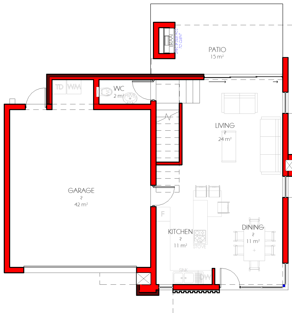
02 GROUND FLOOR 1 : 100
